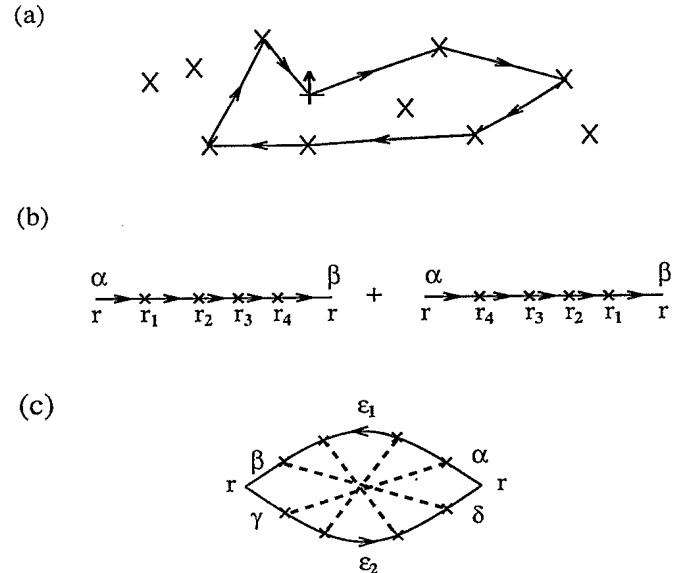
FIG. 1. (a) Schematic path contributing to the local density of states at a Kondo impurity. Even with spin-orbit scattering by impurities (the \times 's), the equal weighting of time-reversed paths (b) guarantees a diagonal single-particle propagator G_{\beta\alpha}(r,r) , which preserves the Kondo effect. (c) The cooperon contribution, \langle G_{\beta\gamma}^a(r,r;\epsilon_2) G_{\beta\alpha}^r(r,r;\epsilon_1) \rangle , to the disorder-averaged two-particle propagator, \langle \Pi_{\alpha\beta\gamma\delta}(r,r;\epsilon_1,\epsilon_2) \rangle .
