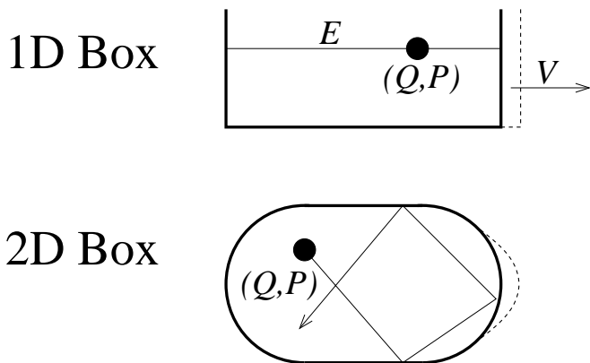
FIG. 2: A ‘gas’ particle in a box is driven by moving the wall. This is essentially the same as Fig.1c, but now the moving wall is not regarded as a dynamical entity. (a) illustrates the case of one-dimensional box, while (b) is for chaotic box. (Hence, in the latter case, the box should be at least two-dimensional).
