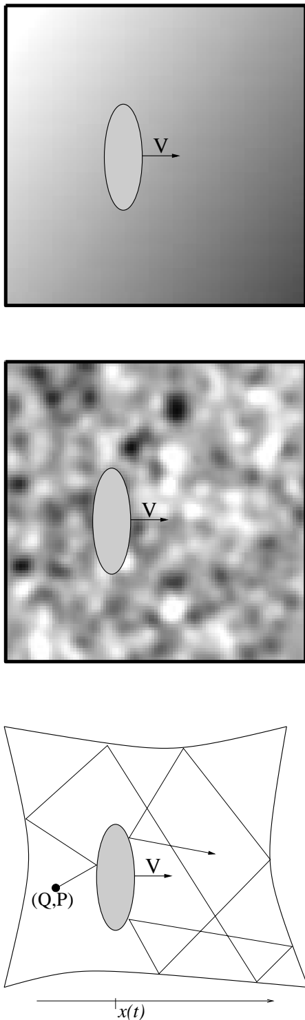
FIG. 1: (a) The Brownian particle in the ZCL model experiences a fluctuating homogeneous field of force. (b) In case of the DLD model the fluctuating field is further characterized by a finite correlation distance. (c) The Brownian motion is induced due to the interaction with chaotic degrees of freedom. x(t) is the (classical) position of the Brownian particle.
