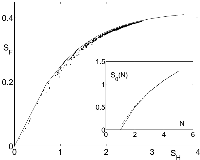
Fig.1: The excess information entropy of a mixed quantum mechanical state S_F versus the von Neumann entropy S_H . The solid line is for uniform mixtures, while the dots are for randomly chosen (nonuniform) mixtures. Inset: The information entropy of a pure quantum mechanical state as a function of the Hilbert space dimension N . See Eq.(8). The dashed line is the asymptotic approximation.
