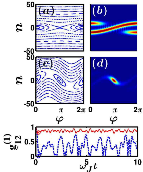
FIG. 3: (Color online) Quantum Kapitza pendulum with vertical driving, and |0, \pi\rangle coherent preparation. The panels are arranged as in Fig. 1. The parameters are u=100 , \Omega=30 , and N=100 . The strength of the driving is q=0 (a,b, lower panel dashed blue) and q=3 (c,d, lower panel solid red). Circles denote the time at which the Husimi distribution in (c,d) is plotted. The classical stabilization of the inverted pendulum results in a protected single-particle coherence of the initial preparation.
