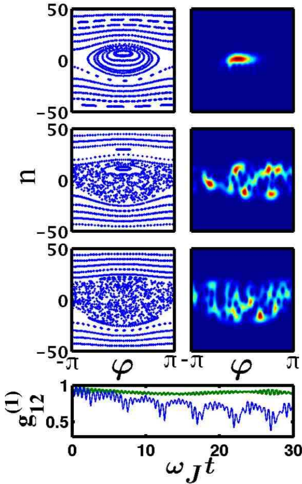
FIG. 2: (Color online) Mean-field stroboscopic phase-space plots of classical trajectories (left), and a representative N=100 many-body quantum Husimi distribution (right), for the dynamics that is generated by the BHH with V_h(t) driving, assuming |0,0\rangle coherent preparation. The parameters are u=30 , and \Omega=1 . The strength of the driving is q=0.1 (top), and q=0.5 (middle), and q=1.0 (bottom). The evolution of the fringe-visibility is plotted in the lower panel for q=0.1 (bold solid, green) and q=1.0 (solid, blue). The circle indicates the time of the Husimi plot.
