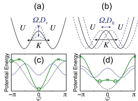
FIG. 1: (Color online) Schematics of a driven Bose-Josephson junction: (a) The ‘vertical’ driving obtained by time-dependent modulation of the barrier height between the wells; (b) The ‘horizontal’ driving is via lateral shaking of the double-well potential; (c) The potential term in the Josephson Hamiltonian without driving (dash-dot), and with vertical driving (solid) which includes the effective potential (dashed). Circles denote stable stationary points whereas ‘x’ denotes instabilities; (d) The same for horizontal driving. It should be noted that ‘vertical’ and ‘horizontal’ refer to the motion of the pendulum axis in the Kapitza analogy, which incidentally match the direction of potential modulation
