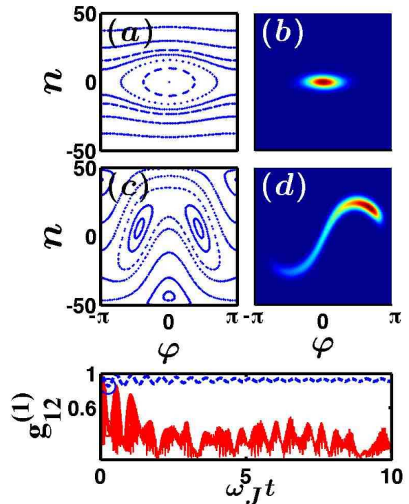
FIG. 4: (Color online) Quantum Kapitza pendulum with horizontal driving, and |0, 0\rangle coherent preparation. The panels are arranged as in Fig. 3, with the same parameters, except u = 30 . One observes the splitting of the ground state. Due to this destabilization the fringe visibility of the preparation is destroyed.
