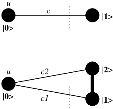
Fig. 1. Toy models that are analyzed in this paper: a particle in a 2 site system (upper illustration), and a particle in a 3 site system (lower illustration). Initially the particle is prepared in the |0\rangle site where it has a potential energy u . The hopping amplitudes per unit time (the c s) are also indicated. In the case of a 3 site system, the time units are chosen such that the hopping amplitude per unit time between |1\rangle and |2\rangle equals unity, while the other amplitudes are assumed to be small ( |c_1|, |c_2| \ll 1 ). The current is measured through the dotted section.
