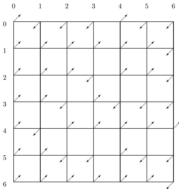
Figure 10.4: Example of a two-dimensional 7 \times 7 lattice with spins pointing either up or down. The variable spin_matrix [1][0] takes the value +1 while spin_matrix [0][6] is -1 .
