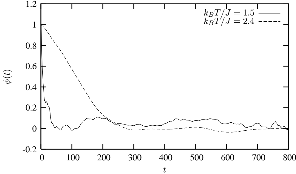
Figure 10.11: Time-autocorrelation function with time t as number of Monte Carlo cycles. It has been normalized with \phi(0) . The calculations have been performed for a 100 \times 100 lattice at k_B T/J = 2.4 with a disordered state as starting point and at k_B T/J = 1.5 with an ordered state as starting point.
