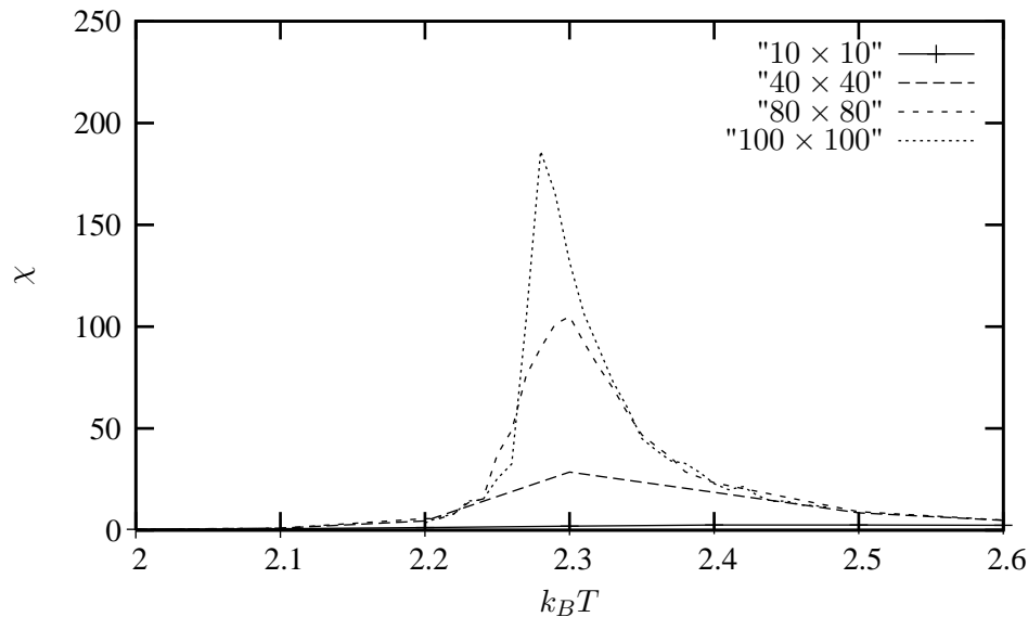
Figure 10.8: Susceptibility per spin as function of the lattice size for the two-dimensional Ising model. Note that we have computed the susceptibility as \xi = (\langle M^2 \rangle - \langle |M| \rangle^2) / k_b T .
