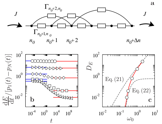
FIG. 1: (a) The network of transitions between states is analogous to a random resistor network. (b) Rate of energy absorption divided by difference in the occupation probabilities of the lowest and the highest states, showing crossover from an initial transient to a steady state. The numerical simulations of (11) employ random-matrix eigenvalues with \beta = 1 , \sigma^2 = 1 , \varrho = 1 , N_p = 3 , and \Phi(\omega) = \varepsilon^2 \exp(-|\omega|/\omega_0)/\omega_0 , for \varepsilon^2 = 1 and \omega_0 = 2 ( \circ ), 1 ( \triangleright ), 0.5 ( \diamond ), 0.3 ( \square ), and 0.25 ( \triangleleft ). The results were averaged over 200 realisations of \hat{\mathcal{H}}_j . The asymptotes are: left, linear-response for the initial transient [eq.(21)], right, steady state determined by network model [eq.(14)]. (c) Energy-diffusion constant D_E vs. \omega_0 . Symbols are long-time asymptotes from figure 1b. The solid line is the semilinear response obtained by solving (14), averaging over 20 realisations. Also shown are linear-response approximation [eq.(21)], asymptote to semilinear-response theory [eq.(22)].
