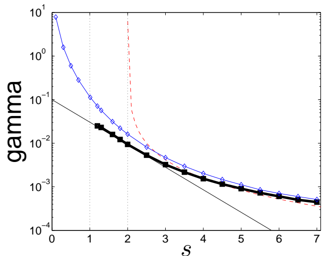
FIG. 3. The inverse localization length \gamma for power-law disorder versus s . Solid line with diamonds is for the non-optimized ( w_{lead} = w_c ) results. Thick solid line with squares is for the optimized ( w_{lead} = w_0 ) results in the range s > 1 , where w_0 is finite. The tangent thin solid line has been fitted in the range 1 < s < 2 where Eq.(6) is expected to hold. The naive Born approximation Eq.(15) is illustrated by dashed line in the range s > 2 . The numerical results here and in the next figures are based on the transfer matrix method (symbols), with several hundreds of realizations up to L \sim 10^4 .
