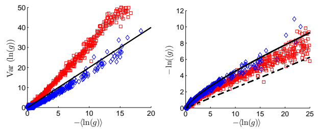
FIG. 6. Testing one parameter scaling for glassy disorder. The variance of \ln(g) (left panel) and the log of the average -\ln(g) (right panel) are plotted against the scaling parameter -\ln(g) . The calculation is done for powerlaw distributed rates with s = 15 (blue diamonds) and s = 1.2 (red squares). The solid line is the standard one parameter scaling prediction for weak disorder, and the dashed line is its asymptotic approximation. One observes that an anomaly develops as the disorder becomes glassy.
