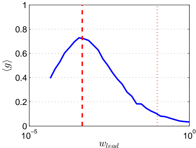
FIG. 2. The average transmission \langle g \rangle as a function of the hopping rate w_{lead} within the leads. The calculation is done for L = 50 disordered samples with conservative log-box disorder \sigma = 10 at k = 0.028\pi . The algebraic and the harmonic mean values of the w_n are indicated by vertical dotted and dashed lines respectively.
