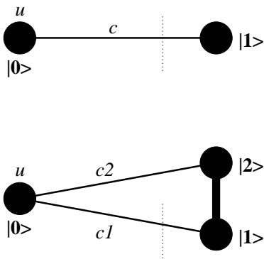
Fig. 1. Toy models that are analyzed in this paper: a particle in a 2 site system (upper illustration), and a particle in a 3 site system (lower illustration). Initially the particle is prepared in the |0\rangle site where it has a potential energy u . The hopping amplitudes per unit time (the c s) are also indicated. In the case of a 3 site system, the time units are chosen such that the hopping amplitude per unit time between |1\rangle and |2\rangle equals unity, while the other amplitudes are assumed to be small ( |c_1|, |c_2| \ll 1 ). The current is measured through the dotted section.
