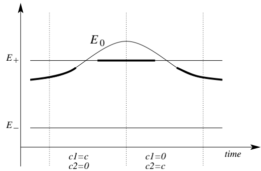
Fig. 2. The adiabatic levels of the 3-site Hamiltonian during one period of a pumping cycle. In the absence of coupling ( c_1 = c_2 = 0 ) the E_0 = u(t) level intersects the symmetric E_+ = 1 level. With non zero coupling these intersections become avoided crossings, and the particle follows adiabatically the thickened lines. For presentation purpose we indicate that either c_1 or c_2 equal zero (“blocked”), but in the general analysis we allow any splitting ratio, including the possibility c_1 = c_2 of having the same amplitude to take either of the two paths.
