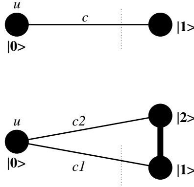
Fig.1. Toy models that are analyzed in the Letter: a particle in a 2 site system (upper illustration), and a particle in a 3 site system (lower illustration). Initially the particle is prepared in the |0\rangle site where it has a potential energy u . The hopping amplitudes per unit time (the c s) are also indicated. In the case of a 3 site system, the time units are chosen such that the hopping amplitude per unit time between |1\rangle and |2\rangle equals unity, while the other amplitudes are assumed to be small ( |c_1|, |c_2| \ll 1 ). The current is measured through the dotted section.
