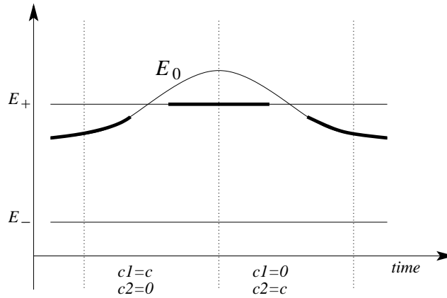
Fig.2. The adiabatic levels of the 3-site Hamiltonian during one period of a pumping cycle. In the absence of coupling ( c_1 = c_2 = 0 ) the E_0 = u(t) level intersects the symmetric E_+ = 1 level. With non zero coupling these intersections become avoided crossings, and the particle follows adiabatically the thickened lines. For presentation purpose we indicate that either c_1 or c_2 equal zero (“blocked”), but in the general analysis we allow any splitting ratio, including the possibility c_1 = c_2 of having the same amplitude to take either of the two paths.
